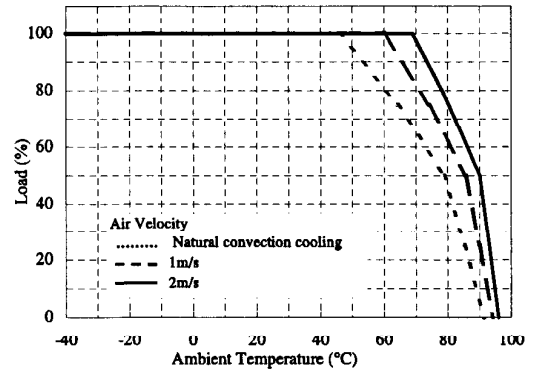
Fig.1-11 PAQ100S48-2R5/B Output Derating at Ambient Temperature (Vin=48V: reference value)
