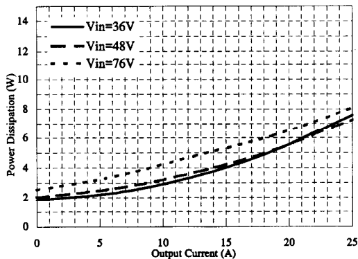
Fig.1-5 PAQ100S48-1R8/B Power dissipation vs Output Current (Output voltage : Nominal, Ta=60°C;typical value)
