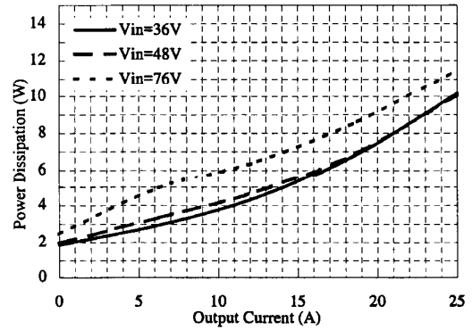
Fig.1-6 PAQ100S48-2R5/B Power dissipation vs Output Current (Output voltage : Nominal, Ta=60°C;typical value)
