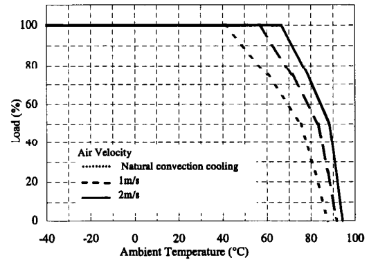
Fig.1-12 PAQ100S48-3R3/B Output Derating at Ambient Temperature (Vin=48V: reference value)
