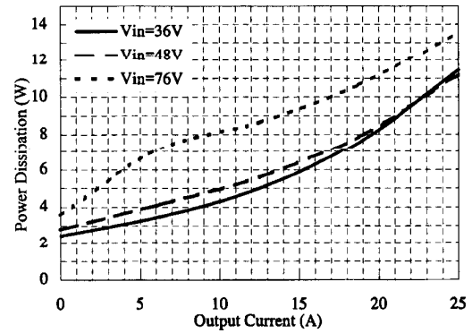
Fig.1-7 PAQ100S48-3R3/B Power dissipation vs Output Current (Output voltage : Nominal, Ta=60°C;typical value)
