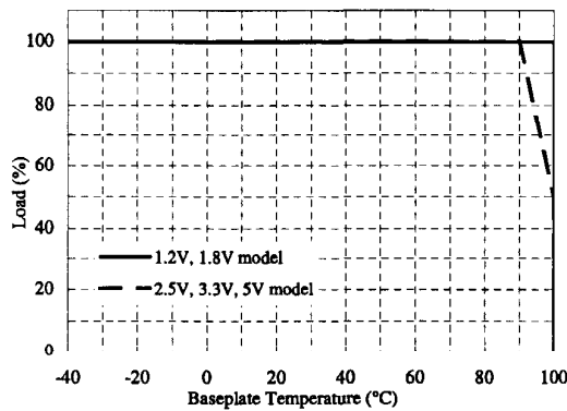
Fig.1-1 PAQ100S48/B Output Derating
