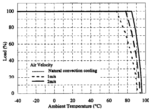
Fig.1-10 PAQ100S48-1R8/B Output Derating at Ambient Temperature (Vin=48V: reference value)
