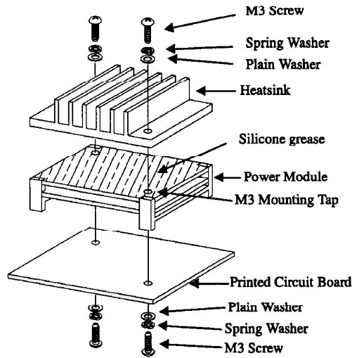
Fig2-1.Installation of Printed Circuit Board and Heatsink
