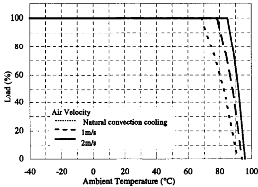
Fig.1-9 PAQ100S48-1R2/B Output Derating at Ambient Temperature (Vin=48V: reference value)
