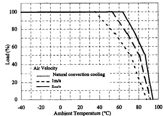
Fig.1-13 PAQ100S48-5/B Output Derating at Ambient Temperature (Vin=48V: reference value)
