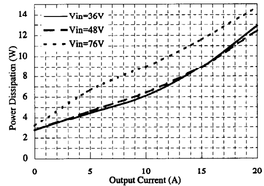
Fig.1-8 PAQ100S48-5/B Power dissipation vs Output Current (Output voltage : Nominal, Ta=60°C;typical value)
