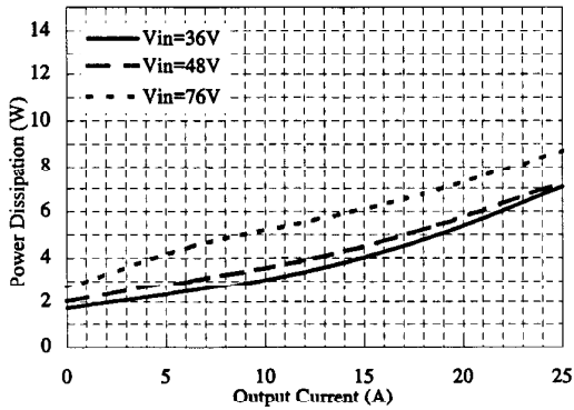
Fig.1-4 PAQ100S48-1R2/B Power dissipation vs Output Current (Output voltage : Nominal, Ta=60°C;typical value)
