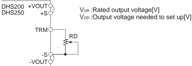
Fig. 4.7 Connection for output voltage decreasing (DHS200/250)
